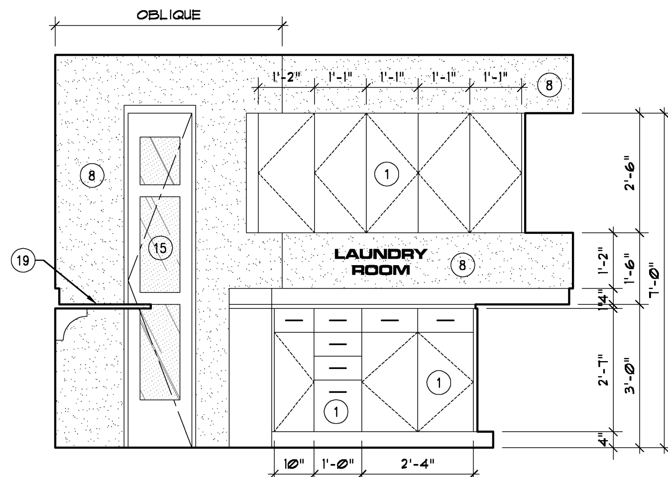
2 INTERIOR ELEVATION SCALE : 1/2" = 1'-0"
