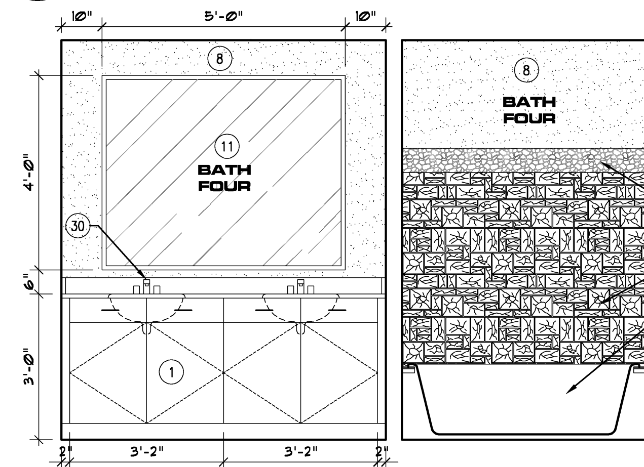
1 INTERIOR ELEVATION SCALE : 1/2" = 1'-0"
