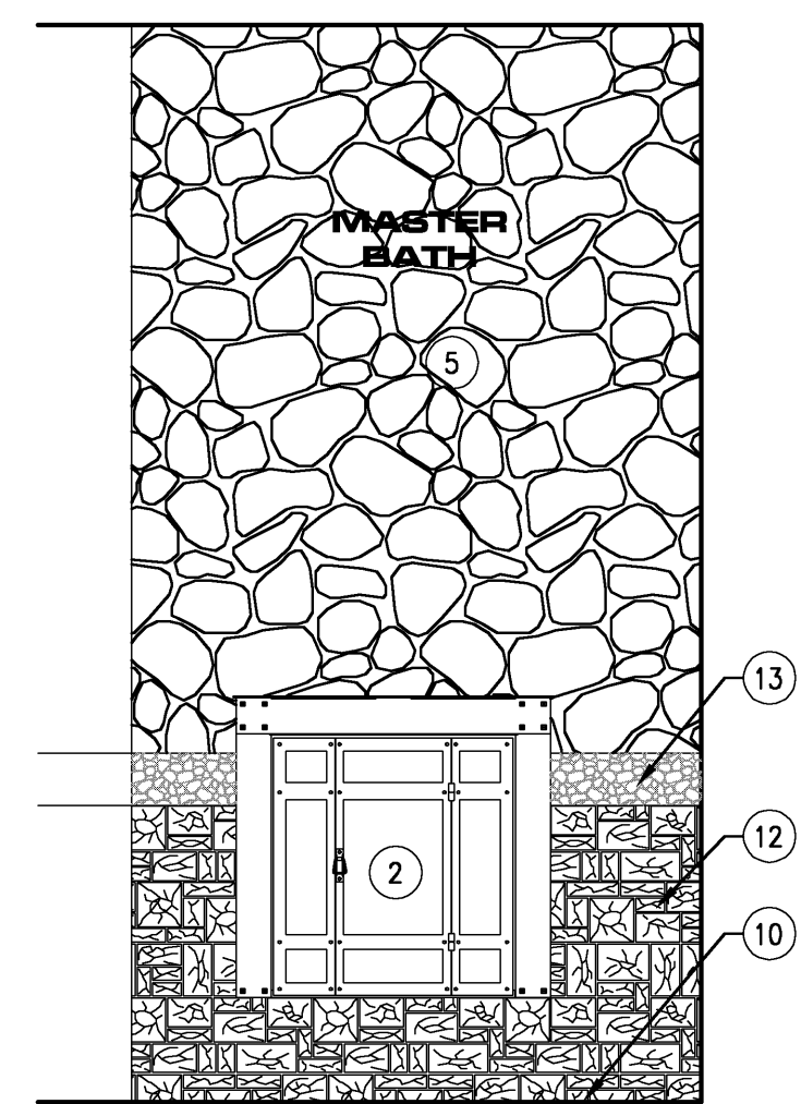
7 INTERIOR ELEVATION SCALE : 1/2" = 1'-0"
