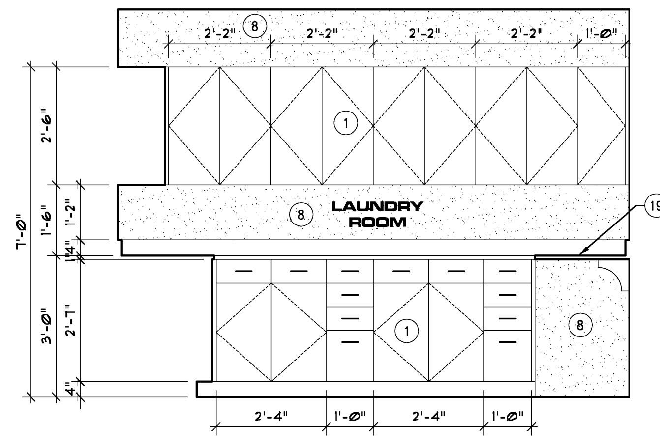
4 INTERIOR ELEVATION SCALE : 1/2" = 1'-0"
